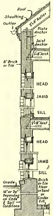
Wall Section
